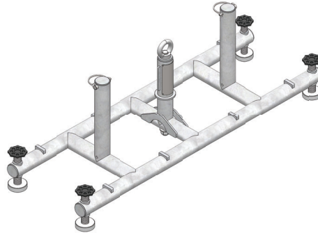
Counterweight Base
