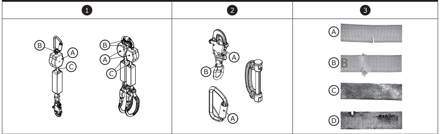
Figure 13 - Energy Absorber Inspection
